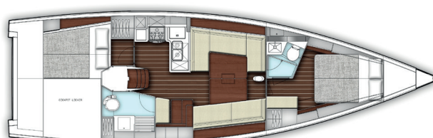
Option 3: 2 cabin/2 heads – available autumn 2017
